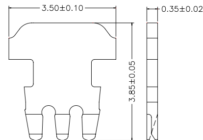
“5”：3 PRONGS FOR STRANDED & SOLID WIRE(S) 多芯線&單芯線用三叉型金片
