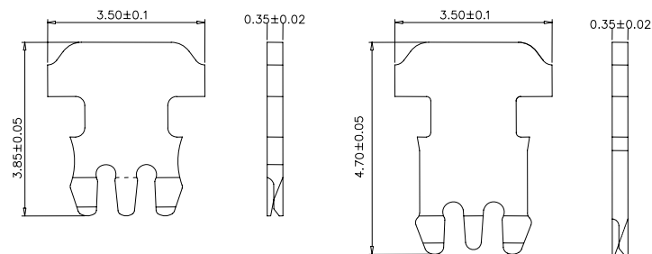
“ ” : 3 PRONGS FOR SOLID & STRANDED WIRE(S) 單多芯線用三叉型金片
