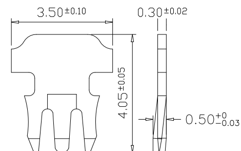
“1”：3 PRONGS FOR SOLID WIRE(S) 單芯線用三叉型金片
