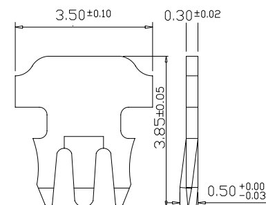
“3” : 3 PRONGS FOR SOLID WIRE(S) 單芯線用三叉型金片
